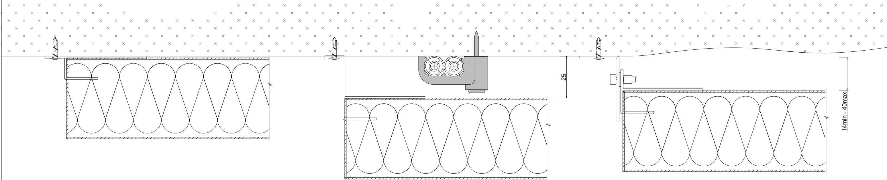
EVEN SURFACES
